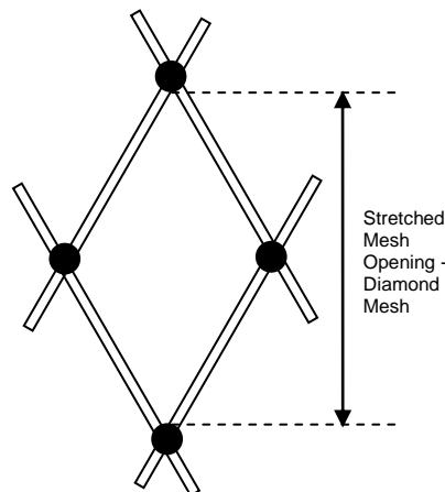
Figure 9-3 Measure stretched mesh opening from the inner edge of knots (modified from (Ferro and Xu 1996)).
