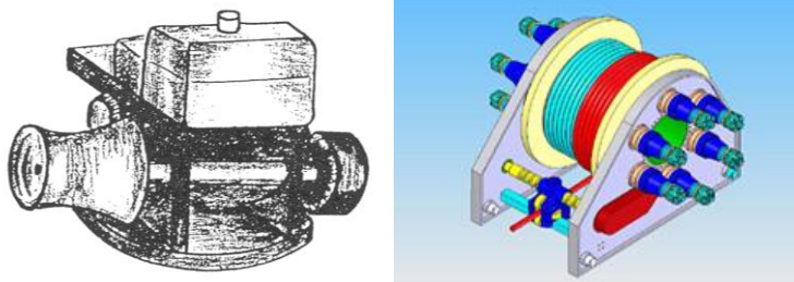
Capstan (left) and purse line winch (right; http://www.cmtwinches.com )
