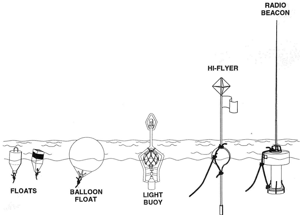
Figure 8-4 Types of floats and buoys. Modified from Hanrahan et al. (1997).
