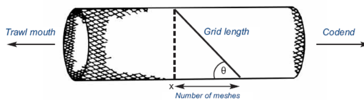
Figure 7-6 Grid angle diagram (Eayrs 2007).
