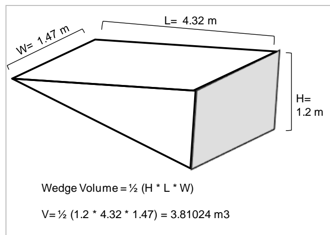
Figure 6-15 Calculation example for wedge volume.
