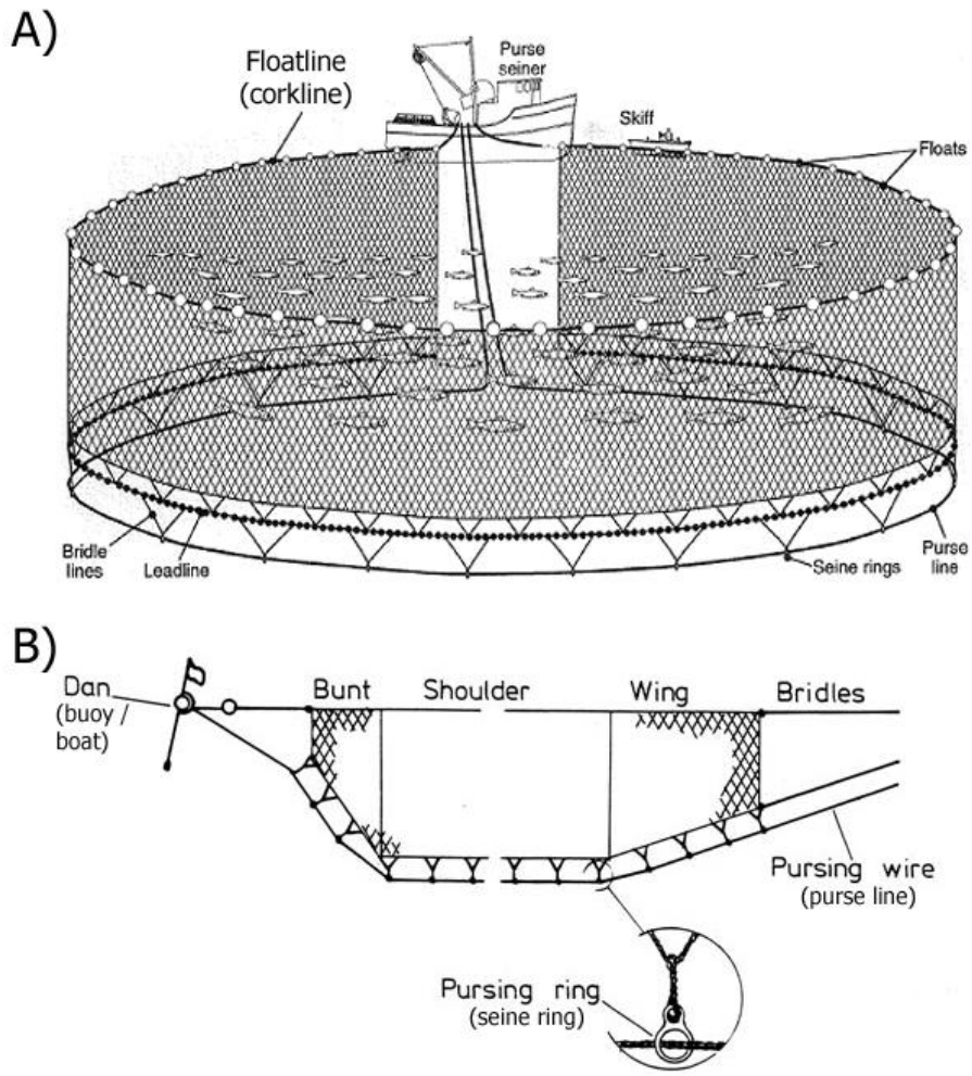
Figure 9-1 Generalized purse seine configuration without (A) and with (B) tapered ends. Images modified from (Hanrahan et al. 1997, FAO 2001-2009).
