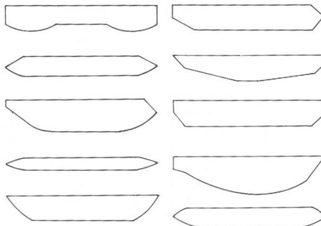
Figure 9-5 Purse seine shapes. Modified from Ben-Yami (1994)
