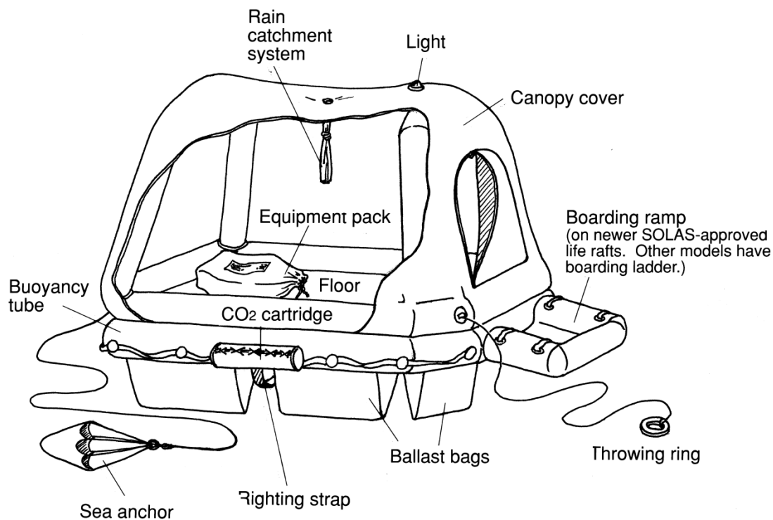
Figure 15-5 Important components of a life raft. Image courtesy of AMSEA.
