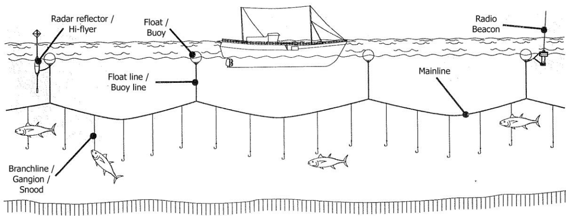
Figure 8-1 Pelagic longline gear components. Modified from Hanrahan et al. (1997).
