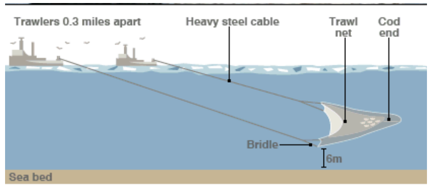
Figure 7-2 Pair trawl – one net pulled by two vessels. Image from http://news.bbc.co.uk/2/low/uk_news/7097257.stm .
