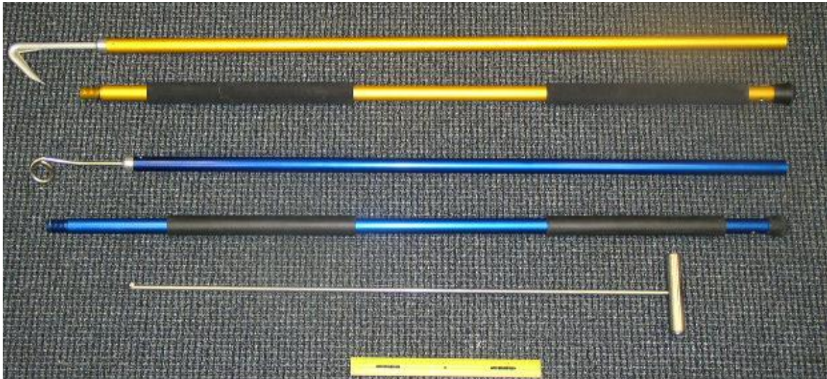
Figure 11-1 Long handled equipment: Line cutter (top), pigtail dehooker (middle) and J-style dehooker (bottom). Images from PIRO (2009).
