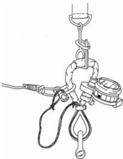
Figure 15-6 Hydrostatic release. Image from AMSEA.
